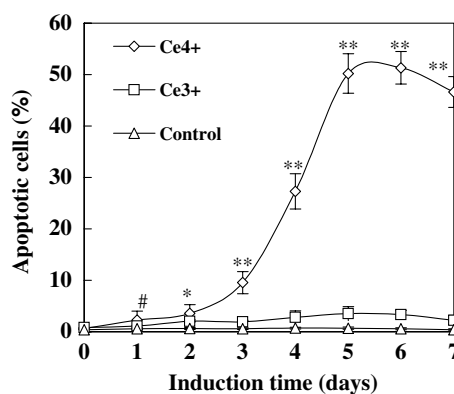
Figure 1. Induction of apoptosis by \text{Ce}^{4+} . \text{Ce}^{4+} of 1 mM and \text{Ce}^{3+} of 1mM respectively were added at 10 day of the cultivation. The percentage of apoptotic cells was estimated using co-staining with Hoechst 33342 and PI, and at least 500 cells were examined in one experiment. Data represent the means \pm S.E.M of three independent experiments. \text{Ce}^{4+} -induced cell compared with the control cell (* P < 0.05 , ** P < 0.001 , # P > 0.05 ).
